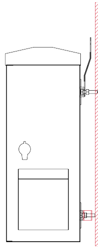
Wall-mounted
