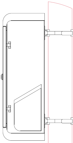
Pole-mounted
