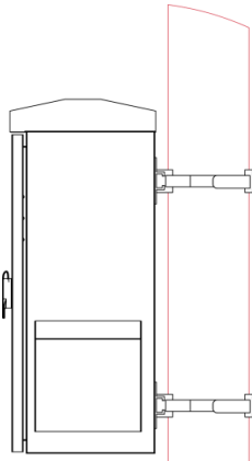
Pole-mounted
